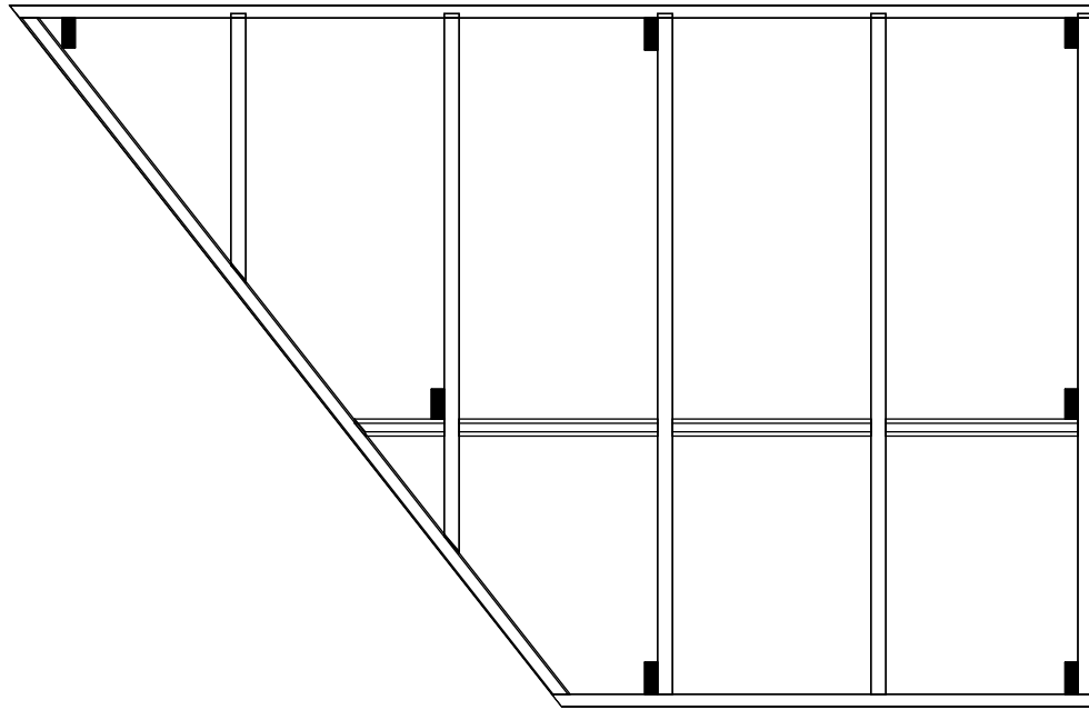
2 LEG PLACEMENT Scale: 1/2" = 1'-0"
